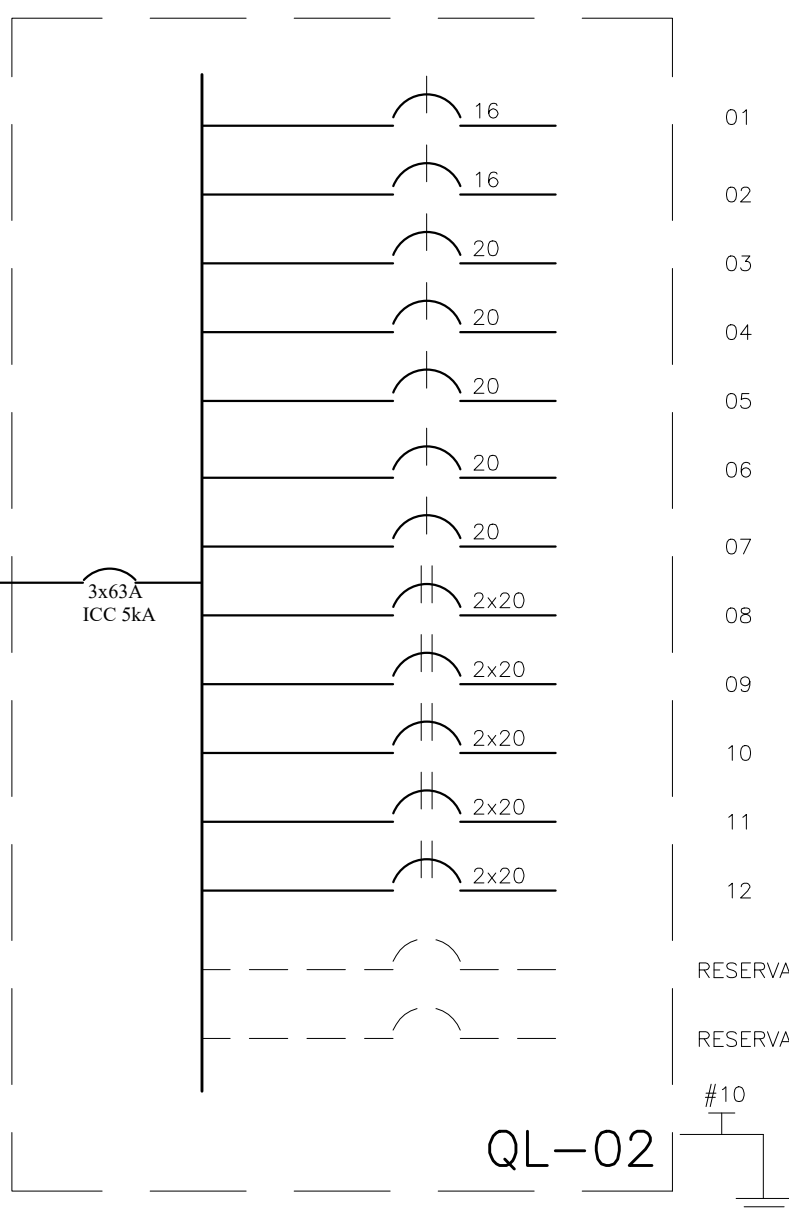
DIAGRAMA UNIFILAR
