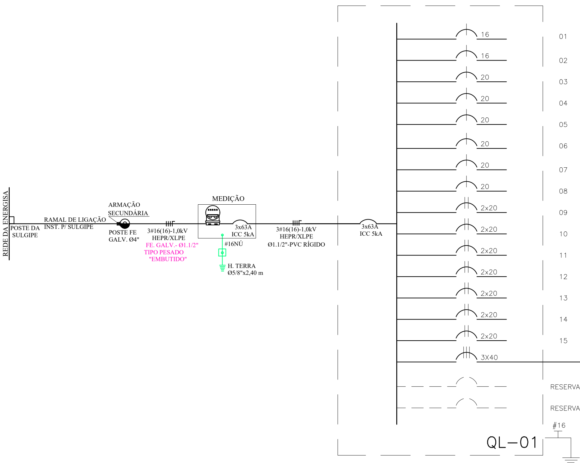
DIAGRAMA UNIFILAR
